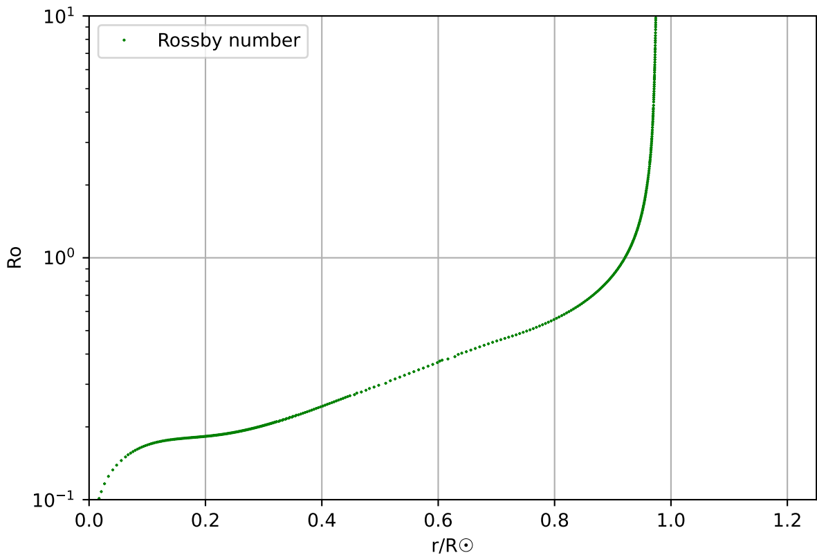
Rossby number, profile 144, age 3.96 \times 10^9
